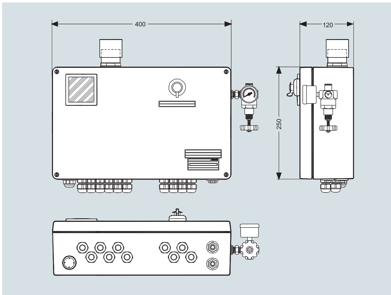
BARTEC purging unit, dimensions in mm
